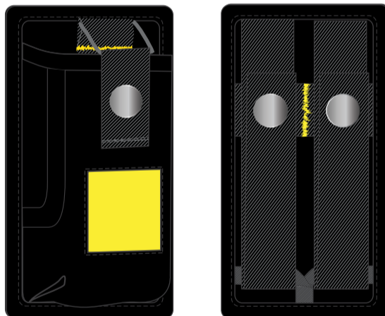
1066745 - Pocket for radio
