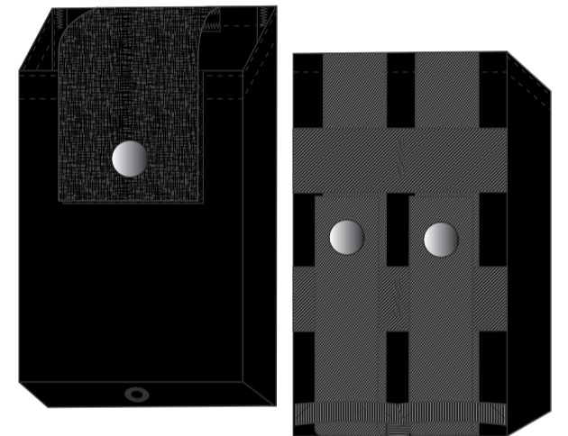
1168728 - Pocket for PLB RESQLINK 400
