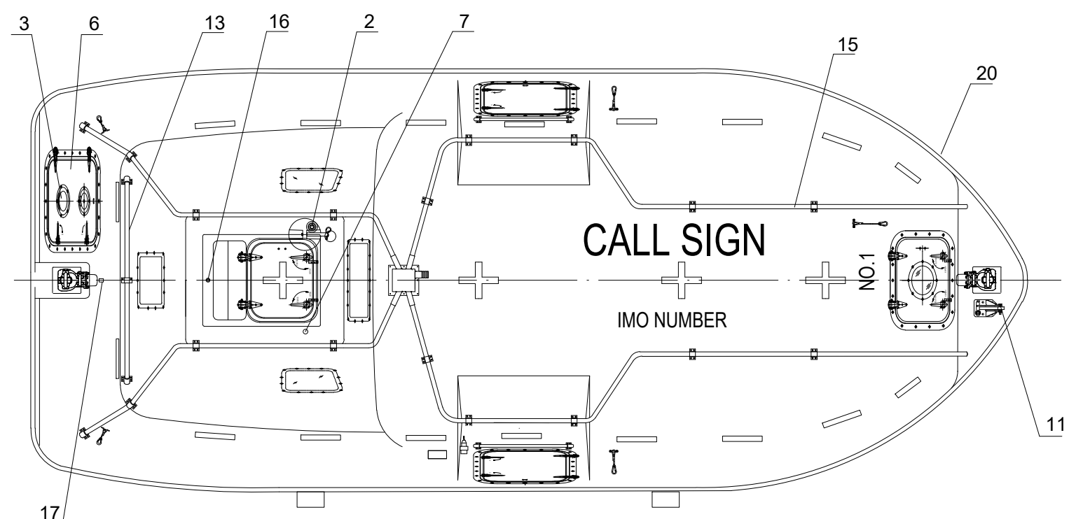
PLAN (BOAT ON PORT SIDE SHOWN, STARBOARD IS MIRRORED)
