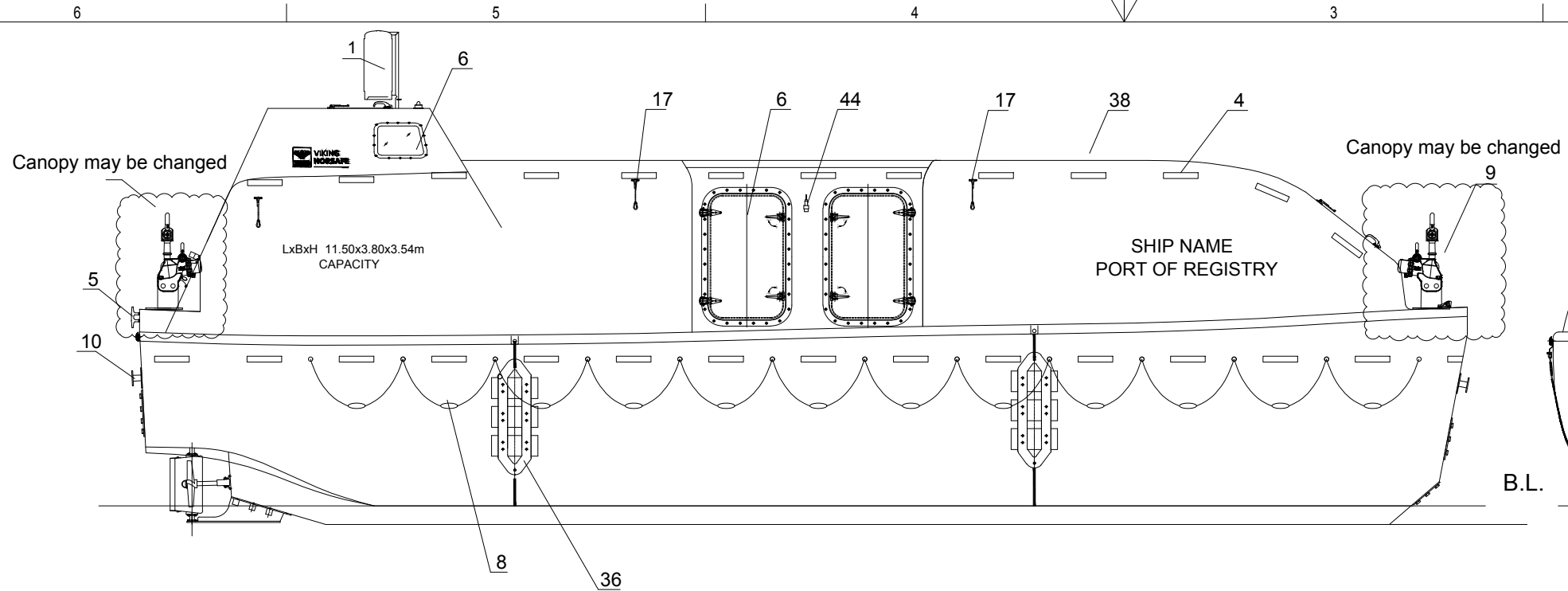
PROFILE
